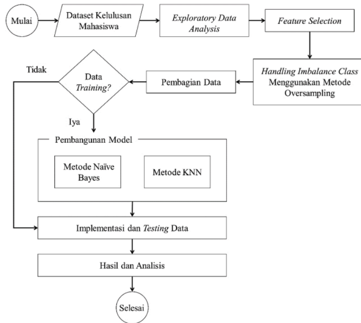
Gambar 1. Flowchart Tahapan Penelitian
