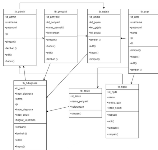
Fig. 2. Class diagram
