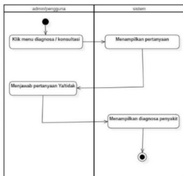
Gambar 2. 6 Activity diagram diagnosa penyakit
