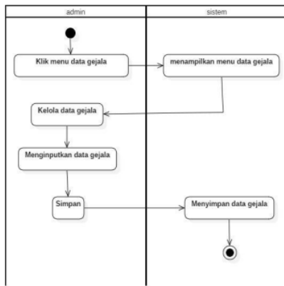
Gambar 2. 5 Activity diagram tambah data gejala
