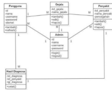
Gambar 2. 7 Class Diagram
