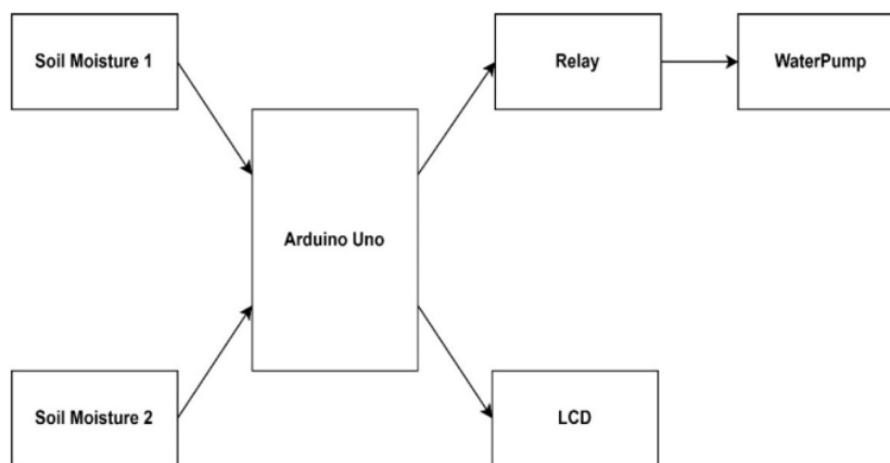
Gambar 1. Blok Diagram
