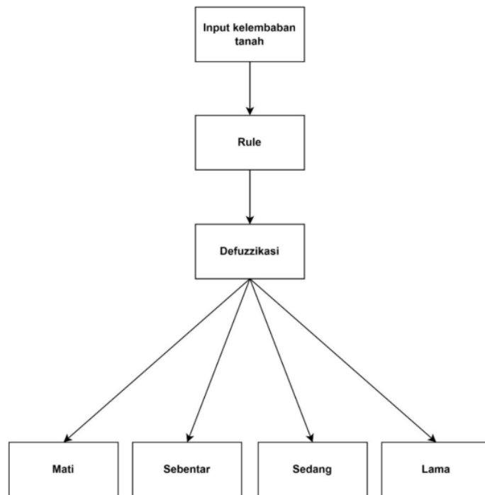
Gambar 5. Fuzzy Logic
