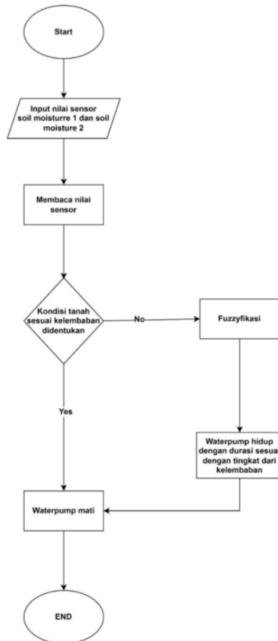
Gambar 2. Flowchart
