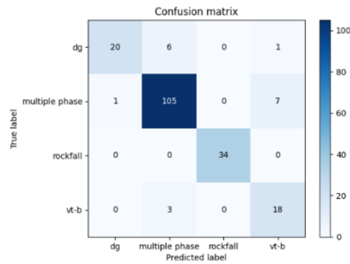
Gambar 6. Hasil Confusion Matrix K=1
