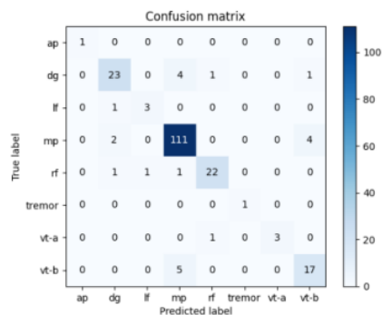
Gambar 8. Hasil Confusion Matrix K=1
