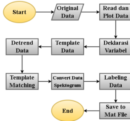
Gambar 2. Preprocessing data
