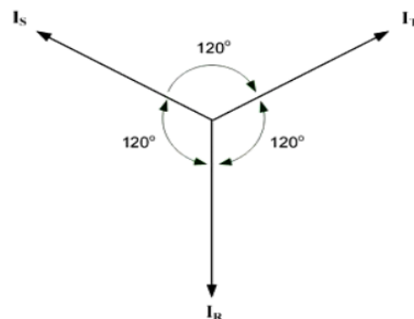
Figure 2. Vector Diagram Balanced Condition
