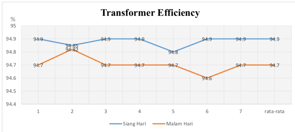
Figure 6. Transformer Efficiency on Supermall Mansion 2, Tower Tanglin
