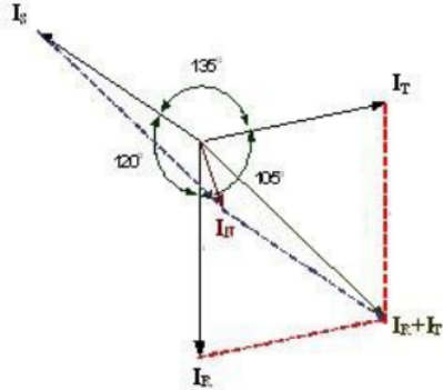
Figure 3. Vector Diagram Unbalanced Condition
