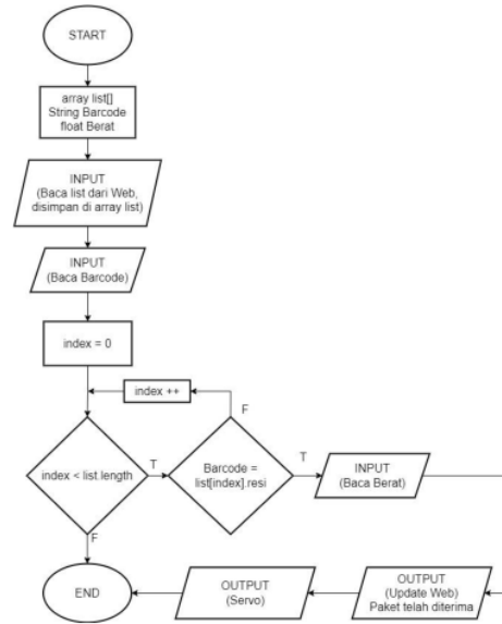
Gbr. 4 Flowchart
