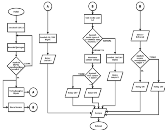
Gbr 9. Flowchart
