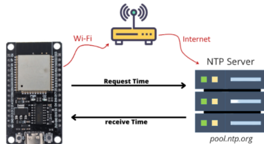
Gbr 3. NTP Server
