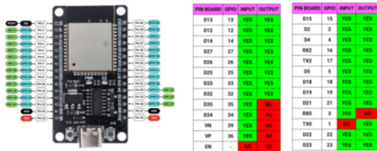
Gbr 2. Pin Board GPIO Number ESP32
