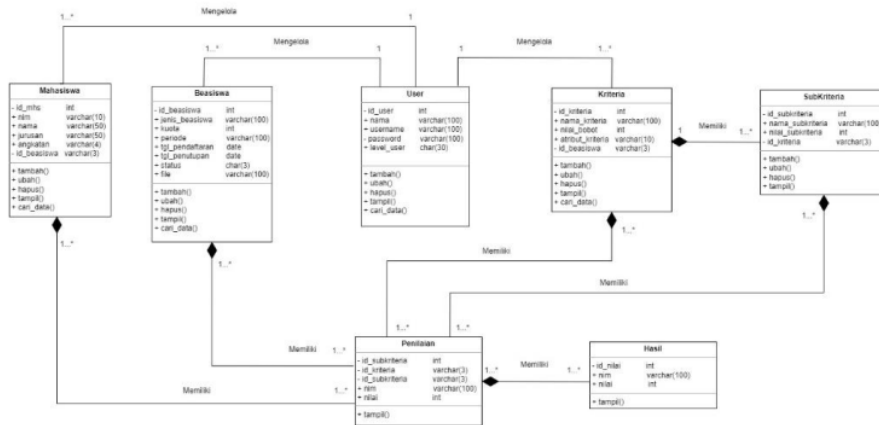
Gambar 3. Class Diagram
