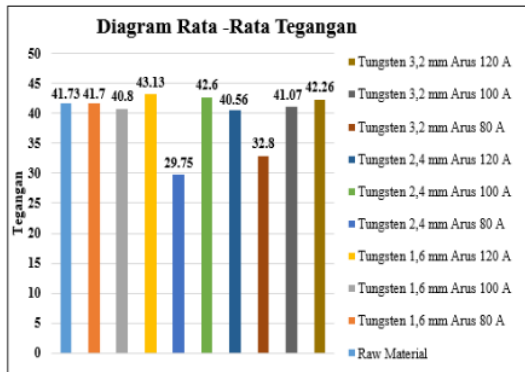
Gambar 25 Diagram Rata – Rata Tegangan
