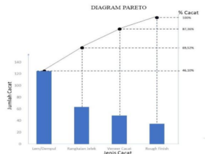
Gambar 3. Diagram pareto
