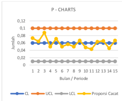
Gambar 5. Peta Kendali P-Chart
