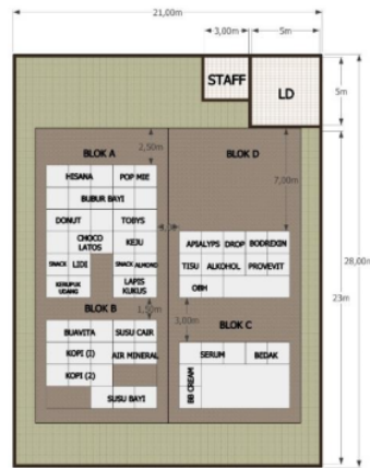
Gambar 1 Layout Awal
