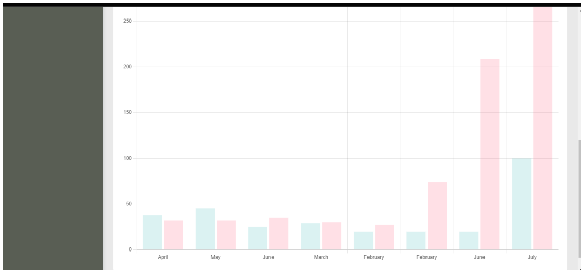
Image 3. 6 Comparison Chart
