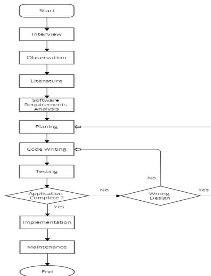
Image 2. 1 Flowchart
