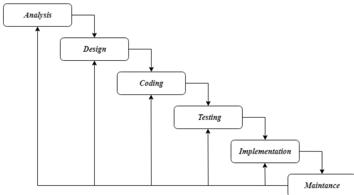
Image 2. 2 Metode Waterfal
