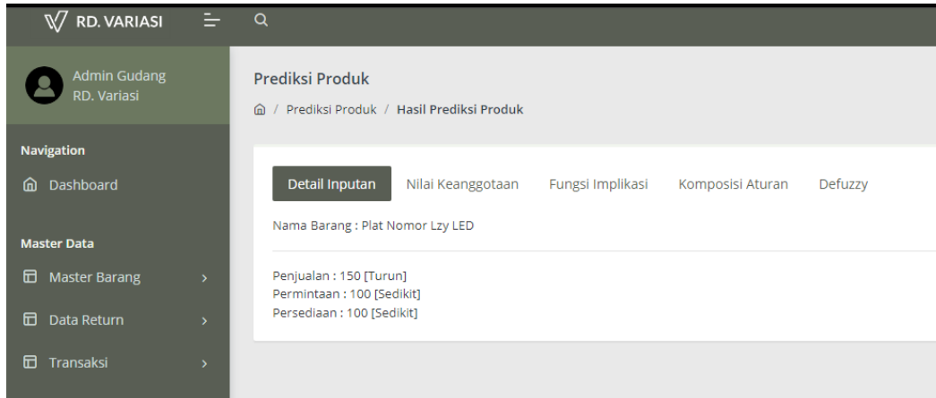
Image 3. 4 Prediction Result
