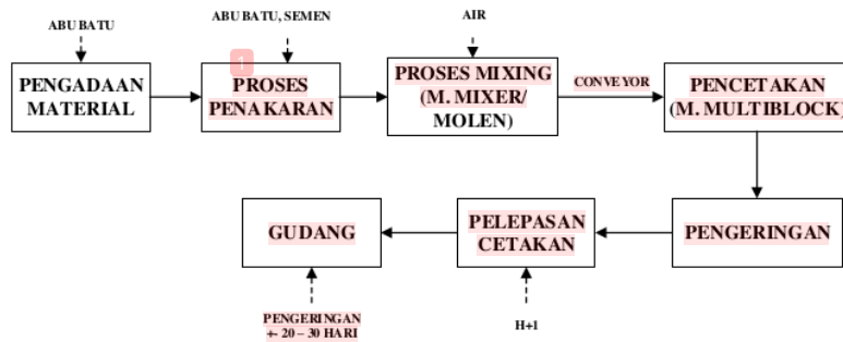
Gambar 2 Proses Produksi Uditch, Box Culvert, Cover
