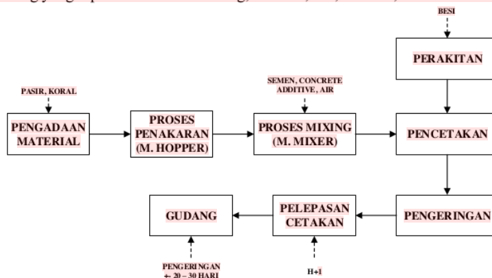
Gambar 1 Proses Produksi Uditch, Box Culvert, Cover
