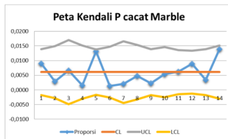
Gambar 8, Peta Kendali Cacat Marble
