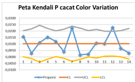
Gambar 5, Peta Kendali Cacat Color Variation
