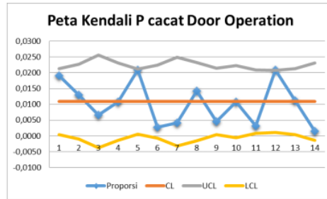
Gambar 6, Peta Kendali Cacat Door Operation
