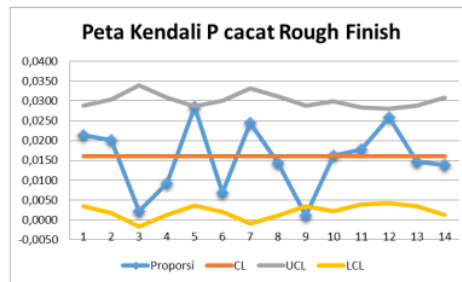
Gambar 7, Peta Kendali Cacat Rough Finish
