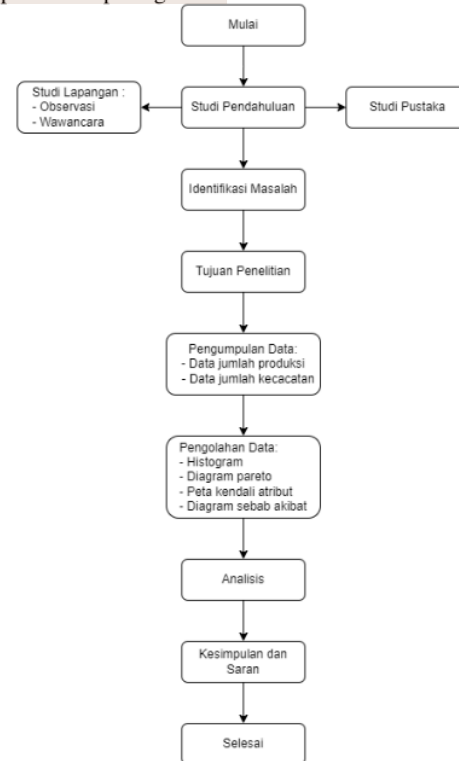
Gambar 1, Flowchart Penelitian
