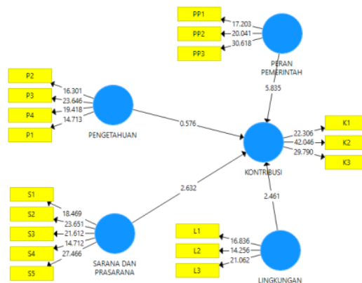
Gambar 6 Diagram Jalur SEM
