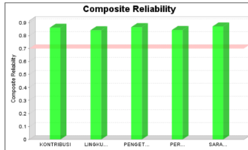
Gambar 9 Nilai Composite Reliability
