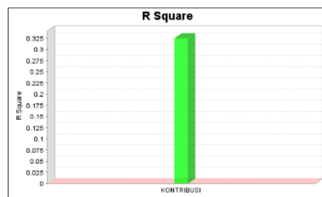
Gambar 11 Nilai R-Square
