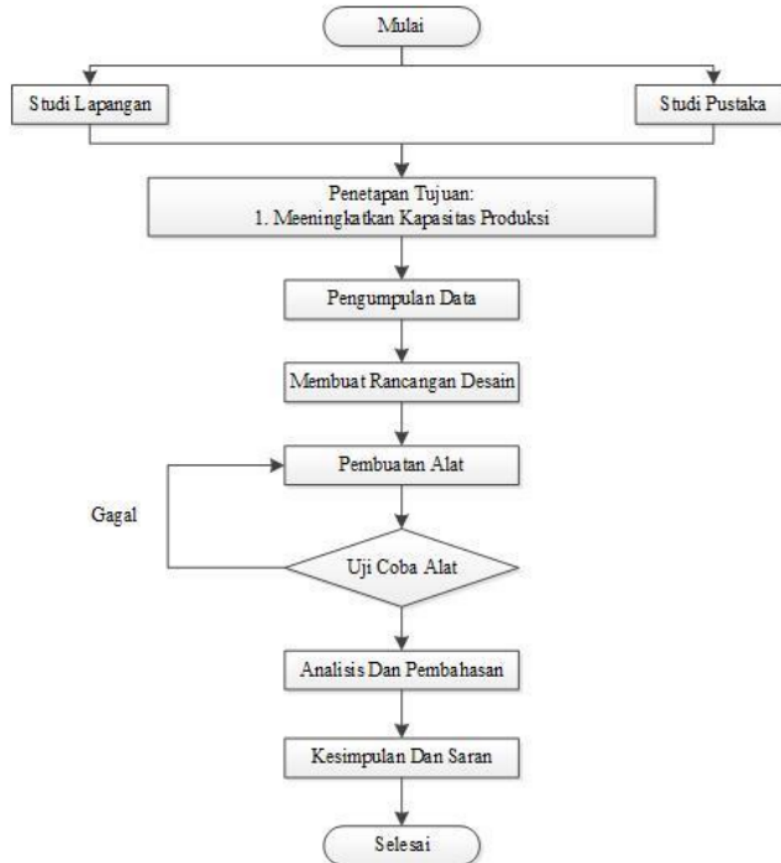
Gambar 1. Flowchat Penelitian
