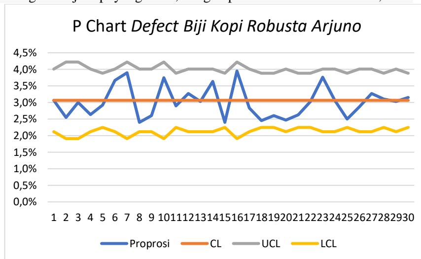
Gambar 2 Peta Kendali P Chart
