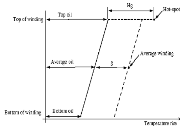
Figure 1. Thermal transformer diagram
