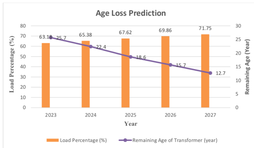
Figure 2. Age Loss Prediction Graph of a Transformer.
