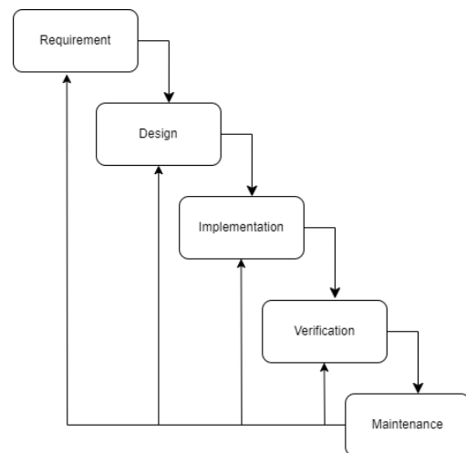
Gambar 2. Model Waterfall
