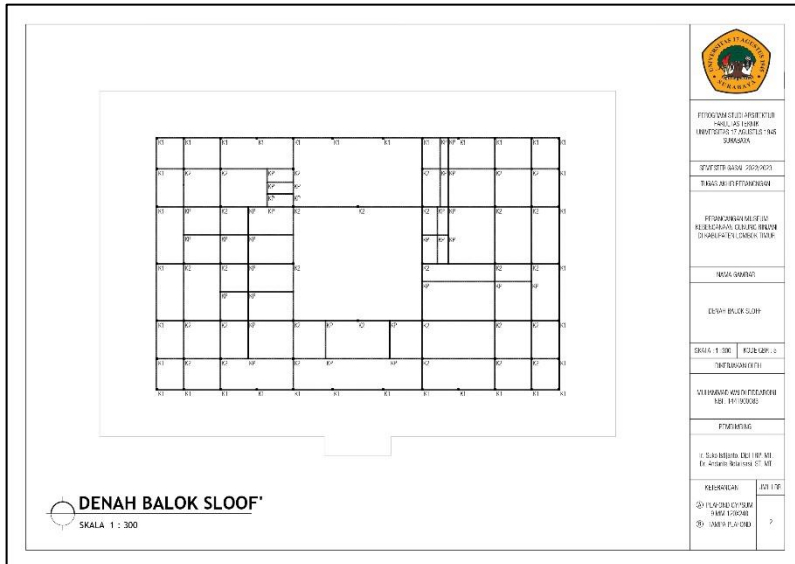
Lampiran 3 denah balok sloof Sumber : Analisis, 2023
