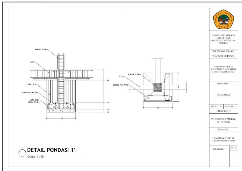
Lampiran 2 detail pondasi
