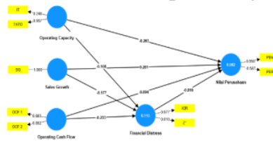
Gambar 1 Convergent Validity
