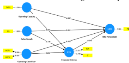
Gambar 2 Re-Convergent Validity
