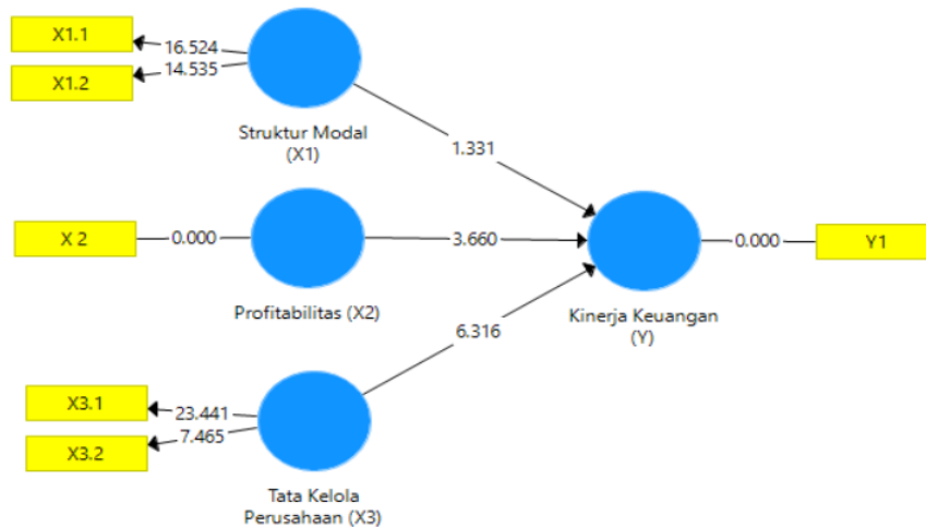
Gambar 3 Output Bootstrapping
