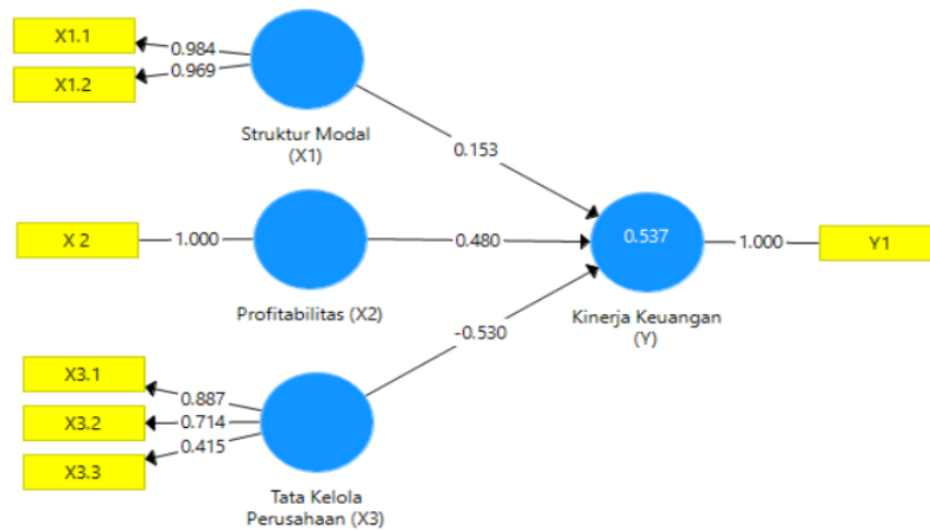
Gambar 1 Outer Loading
