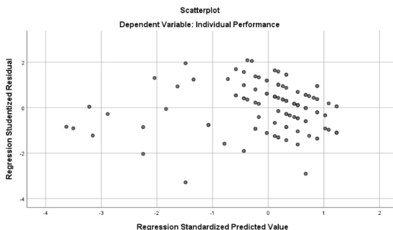
Gambar 2. Uji Scatterplot
