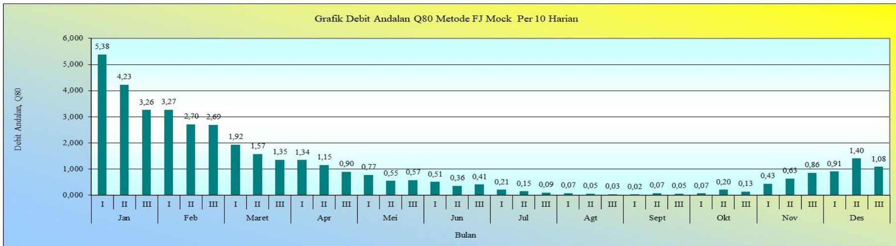
Gambar 4.7 Grafik Debit Andalan Q80 Metode FJ Mock Per 10 Harian
