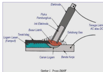
Gambar 1. Proses SMAW
