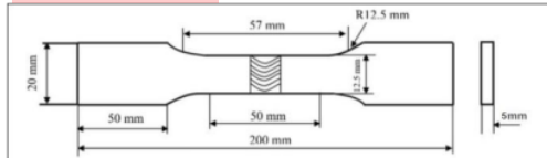
Gambar 2.8 Dimensi Spesimen Pengujian Tarik (ASTM E8)
