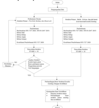
Gambar 3 Diagram alir penelitian
