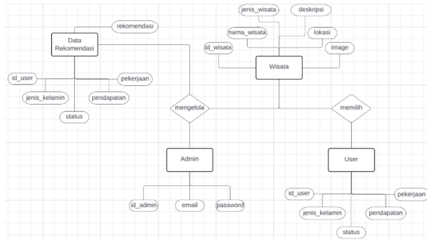
Gambar 3. Entity relational diagram
