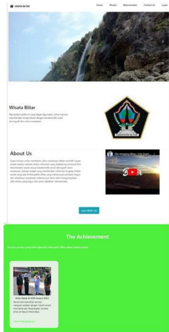
Gambar 6. Halaman home
