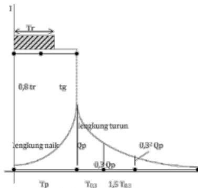
Gambar 2.1 HSS Nakayasu
