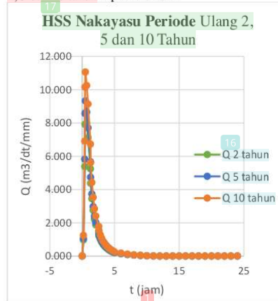
Gambar 4.1 Perbandingan debit banjir HSS Nakayasu
