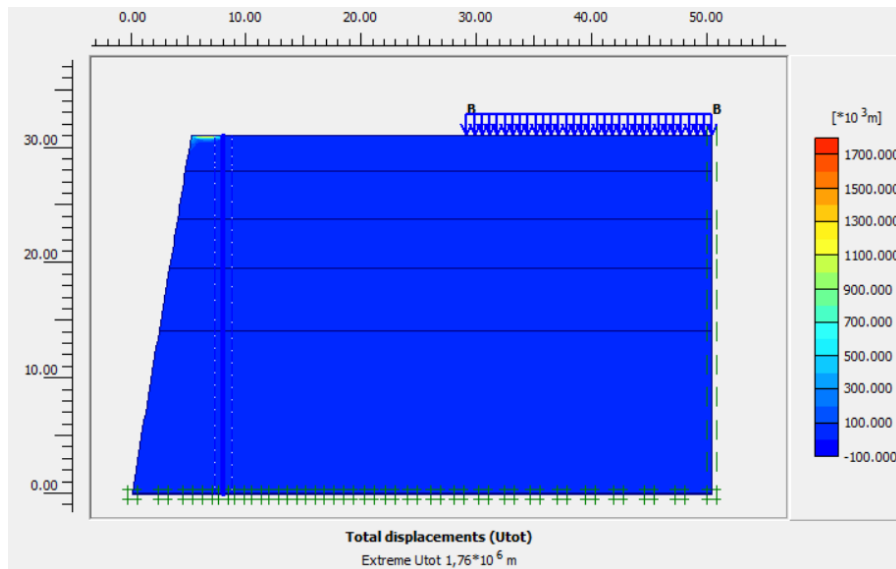
Gambar 14 Perpindahan Total
