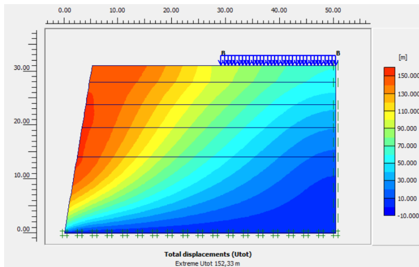
Gambar 8 Perpindahan Total
