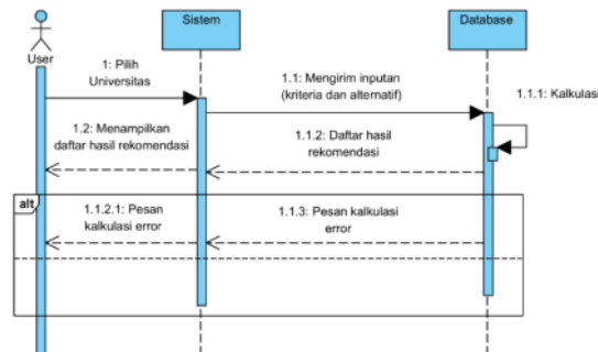
Gambar 2. 3 Sequence Diagram Kalkulasi
