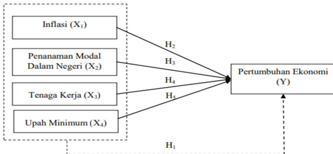
Gambar 1 Model Analisis
