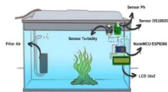
Gambar 2 Implementasi smart aquarium
