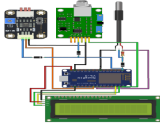
Gambar 6 Rangkaian Hardware
