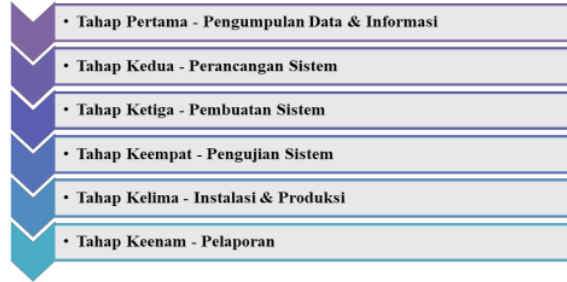
Gambar 1 Alur Penelitian
