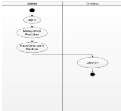
Gambar 6 Activity Diagram
