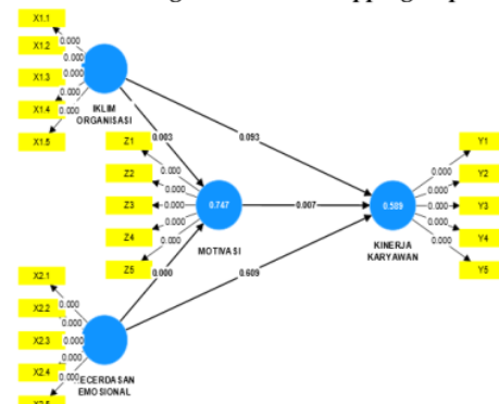
Gambar 4.3 Algorithm Bootstrapping Report
