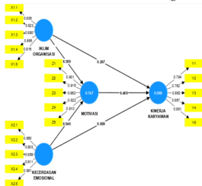
Gambar 4.2 Outer Loading
