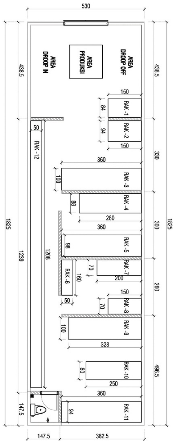
Gambar 3. Layout Usulan
