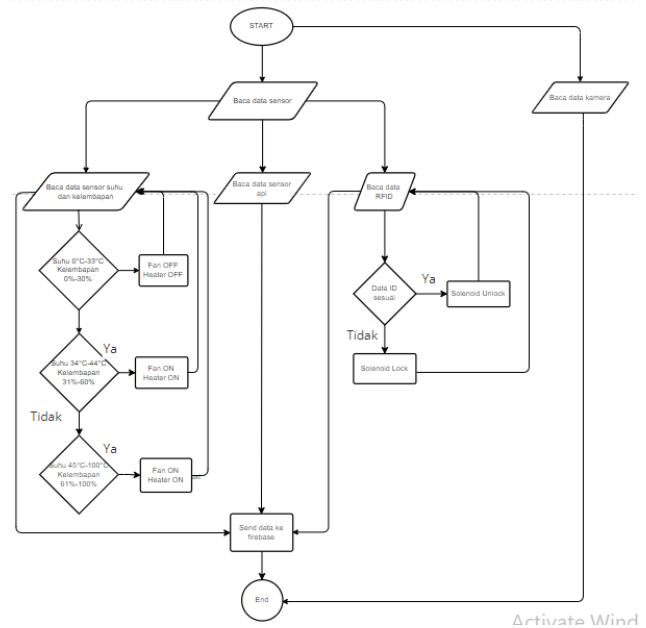
Gambar 6. Flowchart Sistem Arduino
