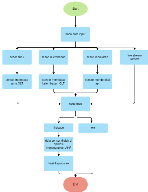
Gambar 5. Flowchart System
