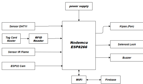
Gambar 4. Blok Diagram
