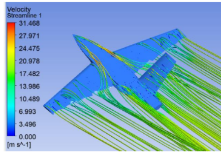
Gambar 32. Velocity Streamline 22 m/s melewati drone baru 15^\circ tampak Isometri
