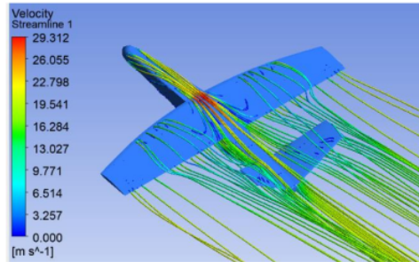
Gambar 26. Velocity Streamline 22 \text{ m/s} melewati drone Airawata 15^\circ tampak Isometri
