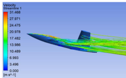
Gambar 30. Velocity Streamline 22 m/s melewati drone baru 15^\circ tampak samping
