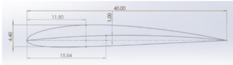
Gambar 3. Airfoil NACA 2411
