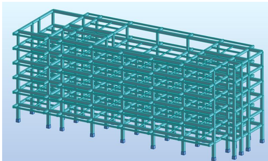
Figure 3 Structural Modelling in Robot Structural Analysis Professional
