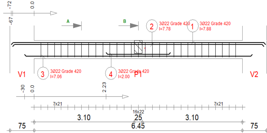
Figure 5 Shear Beam Reinforcement BI2-339
