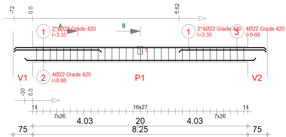
Figure 4 Beam Shear Reinforcement BI1-291
