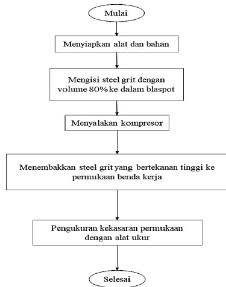
Gambar 2. Diagram alir proses sandblasting
