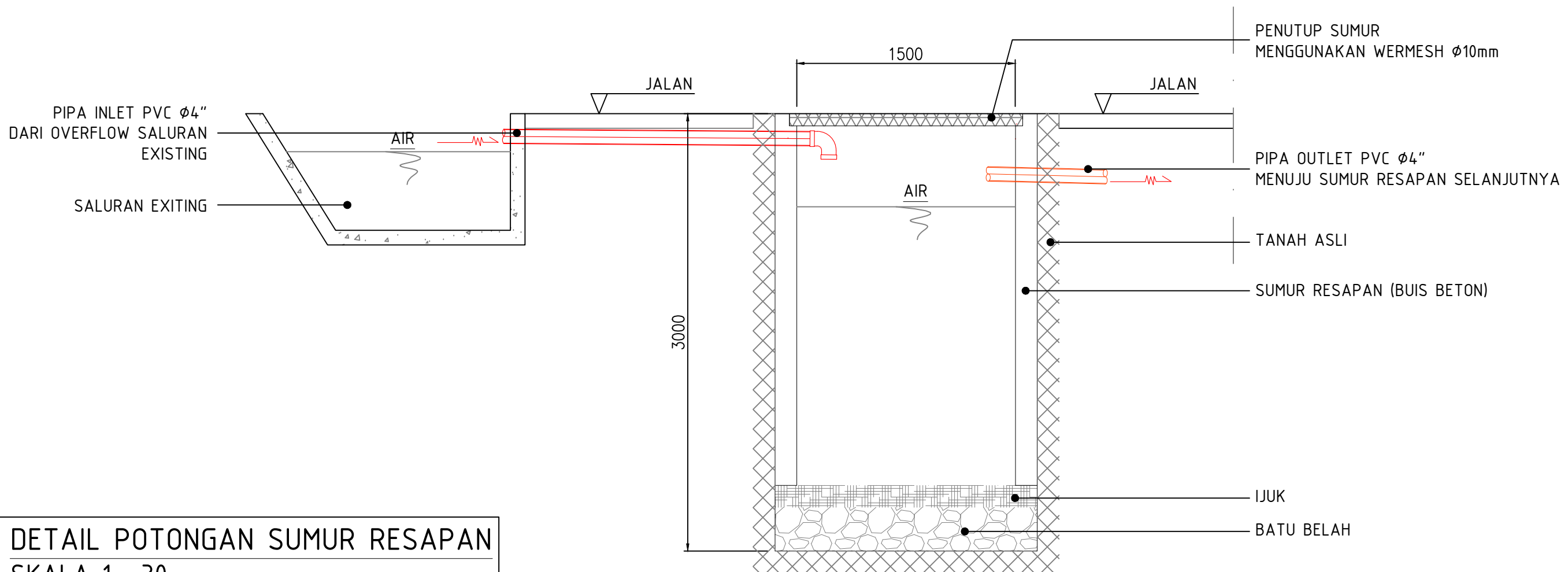
DETAIL SUMUR RESAPAN SKALA 1 : 30
