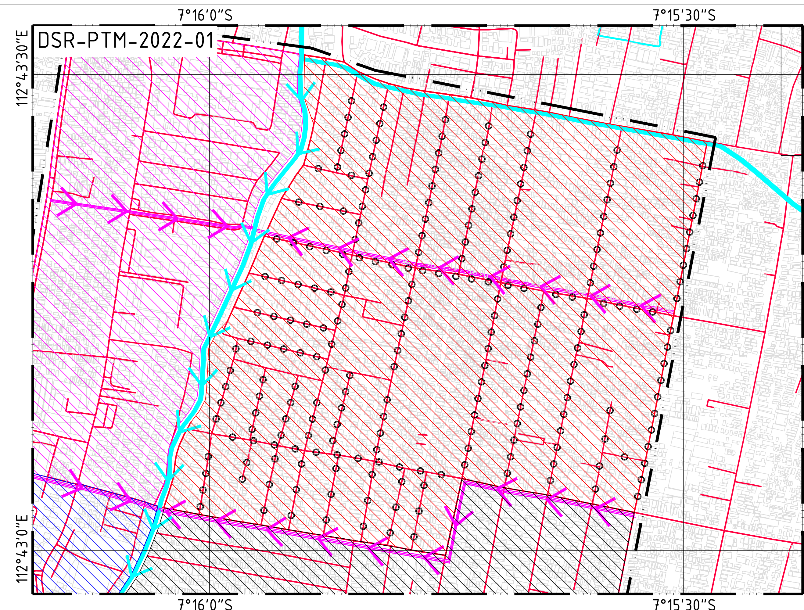
DETAIL LAYOUT SUMUR RESAPAN - SubDAS 1 SKALA 1 : 4500
