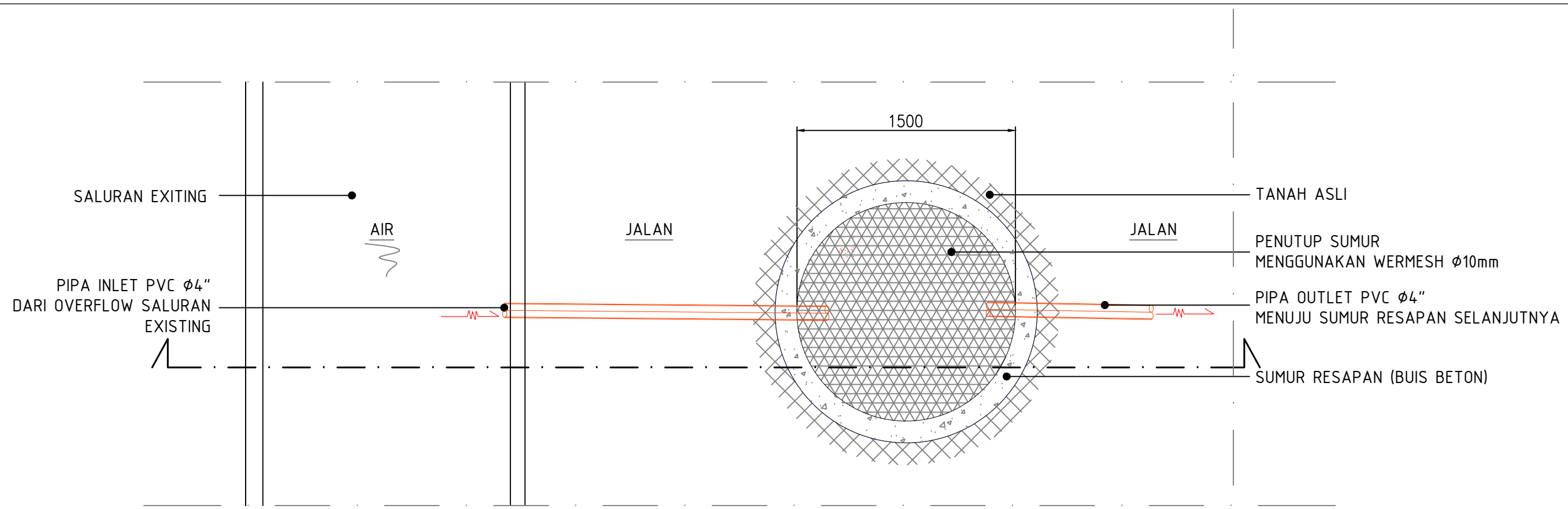
DETAIL SUMUR RESAPAN SKALA 1 : 30
