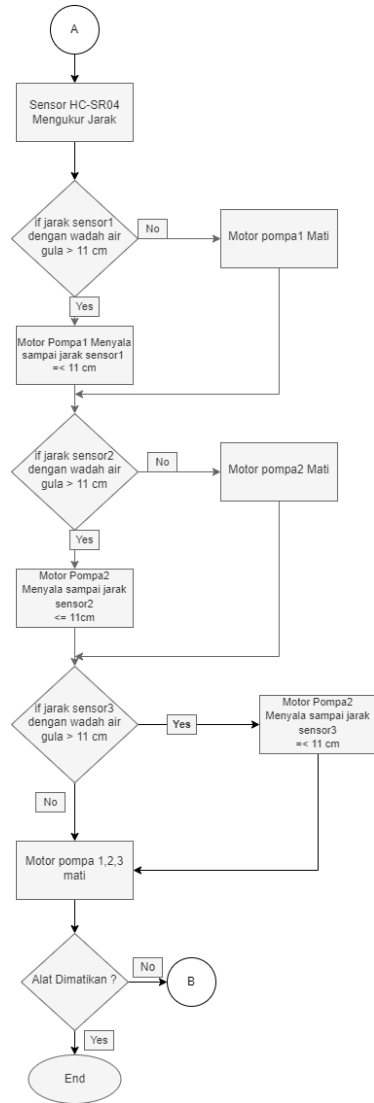
Gambar 2.7 Flowchart Sistem (2)
