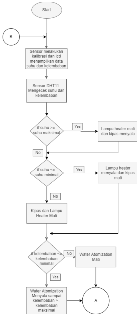
Gambar 2.6 Flowchart Sistem (1)
