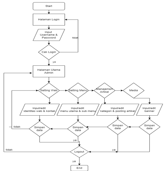
Gambar 3. Flowchart System Admin
