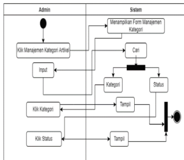
Gambar 7. Diagram activity Category Articles
