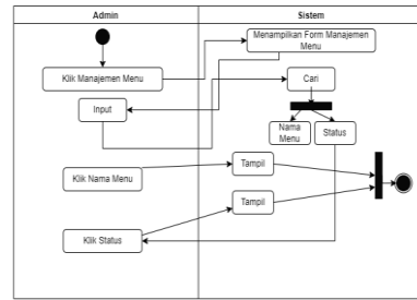
Gambar 9. Activity Diagram Management Main Menu
