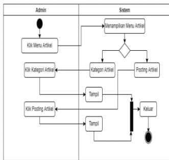
Gambar 6. Diagram activity Menu Articles
