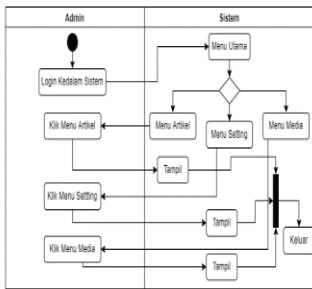
Gambar 5. Diagram activity Main Menu
