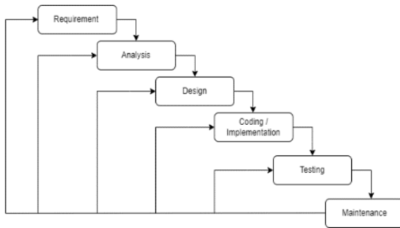
Gambar 1. Waterfall Method
