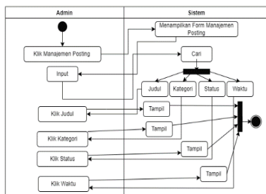
Gambar 8. Diagram activity Posting Articles
