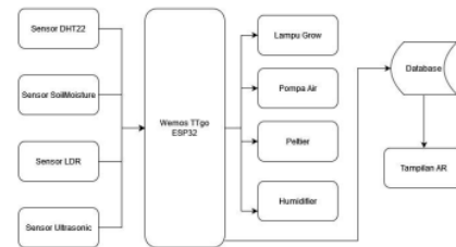
Gambar 4. Blok Diagram
