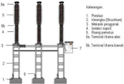
Gambar 2. PMT three pole. [1]
