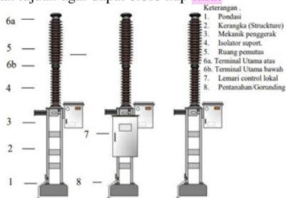
Gambar 1. PMT single pole. [1]
