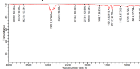
Gambar 3: Hasil FTIR Komposit Volume STK 13% Ukuran 250-300 mesh.
