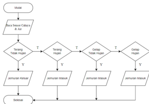
Gambar 3. 3 Flowchart
