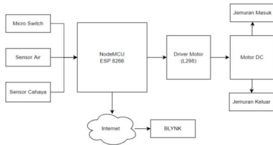
Gambar 3. 1 Diagram Blok
