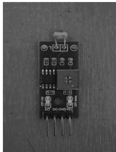
Gambar 2. 3 Sensor Cahaya
