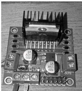
Gambar 2. 5 Driver Motor
