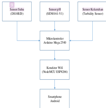
Gambar 2 Blok Diagram
