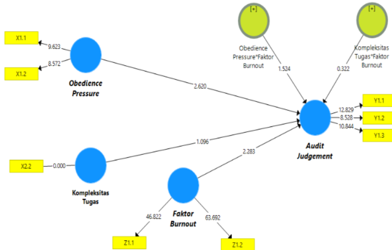
Gambar 2. Uji Inner Models
